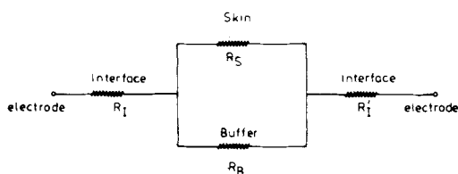
FIG. 3. Electrical model of existing resistances between the electrodes. The R_I and R_I' are equal and represent the resistances of the interface between electrode and buffer medium containing the skin. R_S and R_B are the individual resistances of the skin and the buffer medium ( R_I and R_I' \gg R_B ), respectively.
